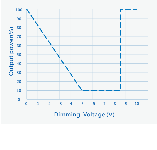
输出功率Vs.调光电压 ( 5-0V )
